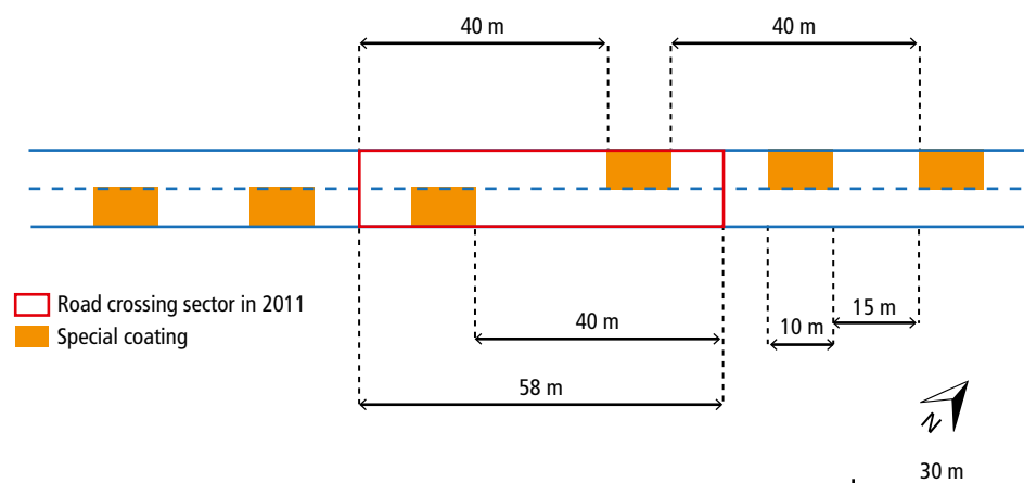
Location of the special coating BBT-M06-CI2 on the RD572.
