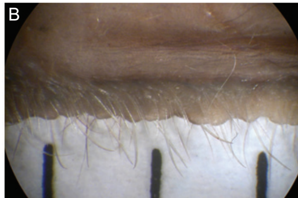
Myotis crypticus sp. nov. EBD 26174
